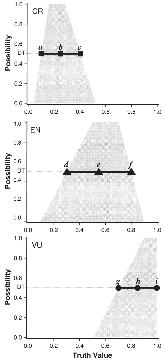
Figure 3. An example of the three fuzzy numbers, which are the result of the rule sets for classifications of critically endangered (CR), endangered (EN), and vulnerable (VU), calculated according to the IUCN rules and methods described in the Appendix. Dispute tolerance (DT) determines the level (represented by the horizontal line) to be used in determining the degree of threat. The bottom of each fuzzy number represents the case that includes all possibilities (DT = 0). The top of each fuzzy number represents the case when dispute tolerance is highest (DT = 1). The points of intersection (e.g., a and c for CR) with the DT line and the middle point (e.g., b for CR) are used in Fig. 4.
