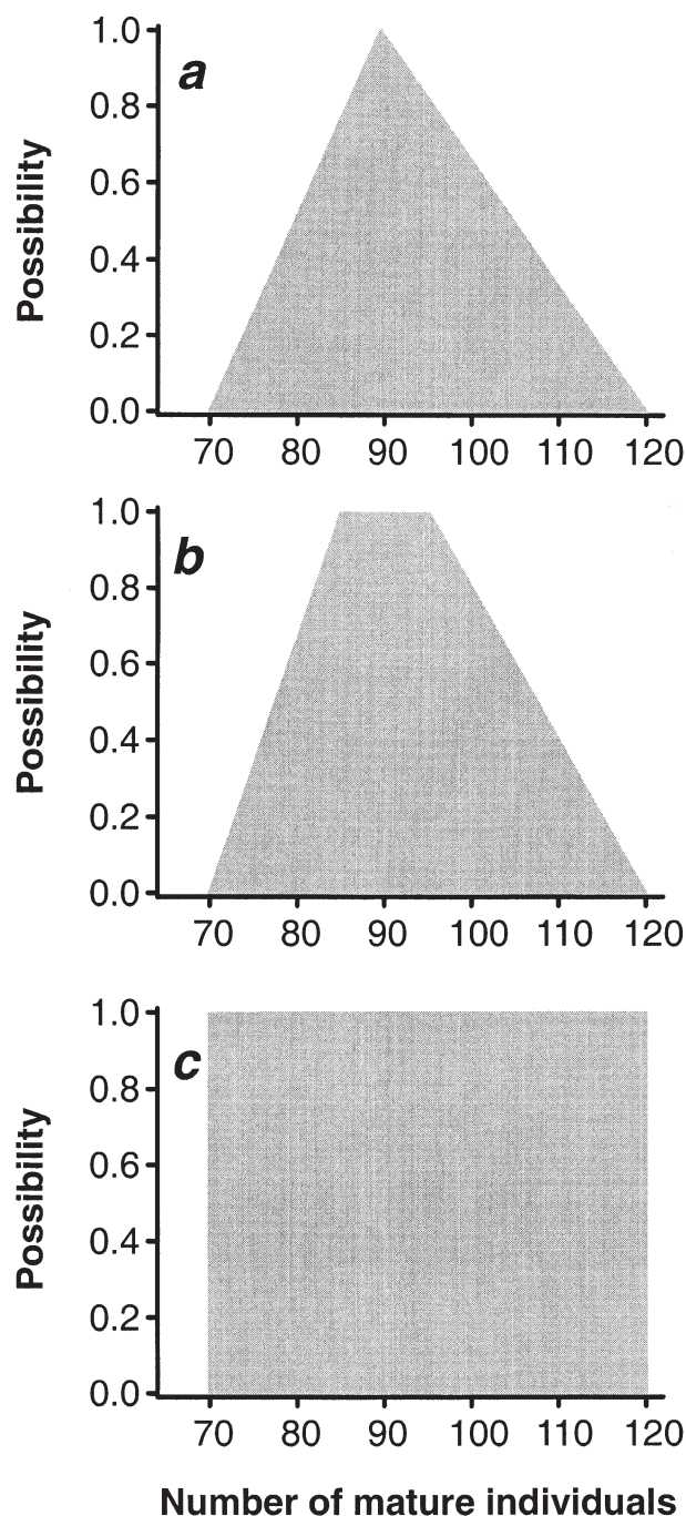
Figure 1. Examples of (a) triangular, (b) trapezoidal, and (c) rectangular fuzzy numbers for the number of mature individuals of a species.
